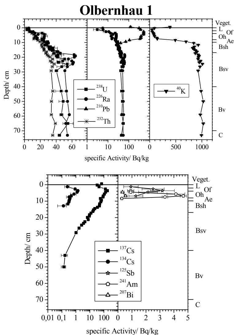
Figure 1: Distribution of natural (above) and artificial radionuclides at sampling site Olbernhau 1. The soil horizons are classified at the right scale.
