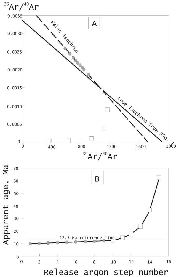
Figure 3: Argon-argon isotope plot (A) and age spectrum (B) for the case, when the activation energy of diffusion for nucleogenic argon 39 lies between those of radiogenic and atmospheric. Intercepts with coordinate axes give distorted results. A locus of points is not a straight line. In the array, filled circles mark a portion exhibited a 'false' isochron. Open squares are omitted from the isochron calculations.
