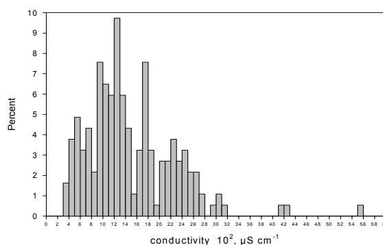
Figure 2: Histogramm of the conductivities in the Historical National Park Troia area (185 data sets).
