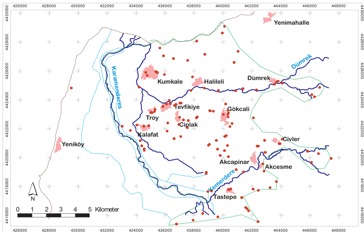
Figure 1: Area of the “Historical National Park Troia” and the locations sampled in 2001 and 2002 (darker dots). Map based on IKONOS data provided by the Troia-Team. Co-ordinates: UTM, WGS84.
