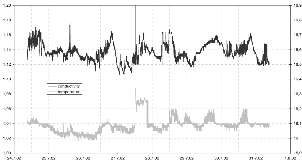
Figure 3: Temperature and conductivity distribution within the Trojan spring cave (conductivity: left scale, upper graph; temperature: right scale, lower graph).
