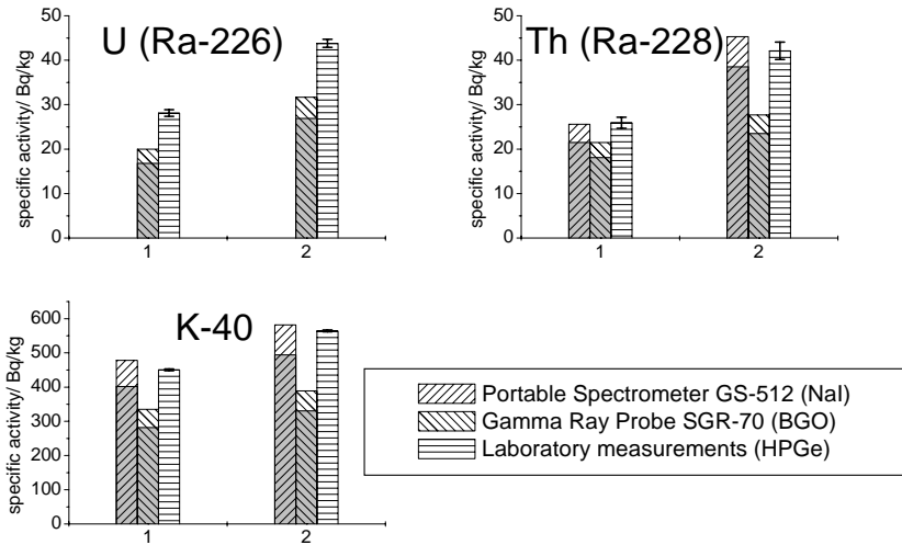
Fig. 6. Comparison of the specific activities of Uranium (top left), Thorium (top right) and Potassium (down left) at the two sampling points on area Hürsingen as measured by different equipments. The laboratory measurements were carried out on dried samples; the values for GS-512 and SGR-70 are corrected to dry soil. Uncorrected contents are marked by grey bars.
