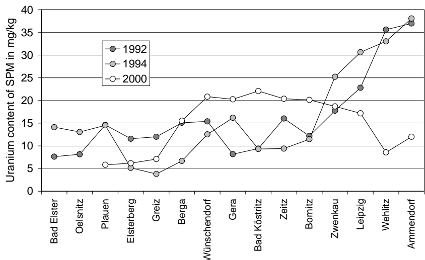
Fig. 3. Uranium contend in SPM 1992,1994 and 2000.
