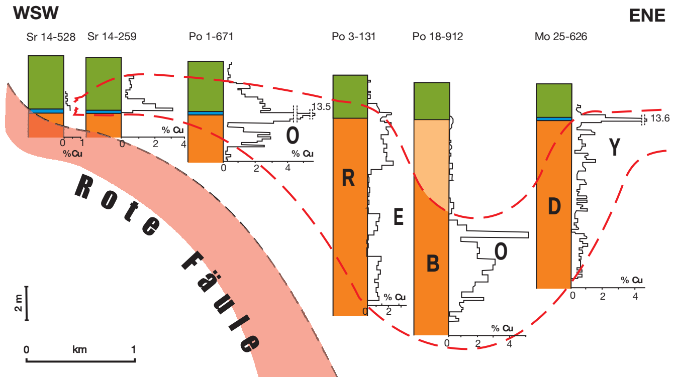
FIG. 6. Simplified cross section through the copper deposits of the Sierszowice, Polkowice, Rudna, and Lubin mines within the Fore-Sudetic monocline, showing the thickness and strong vertical variation of the position of the ore zone relative to stratigraphy (adapted from Wodzicki and Piestrzyński, 1994).
