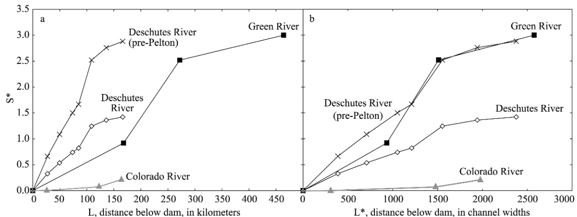
Figure 4. Longitudinal trajectories of change in S^* for the Green, Colorado, and Deschutes Rivers below Flaming Gorge, Glen Canyon, and Pelton-Round Butte dams, respectively. Two trajectories are shown for the Deschutes, depending on whether the reference value for the above-dam sediment flux is calculated as pre- or post-upriver dam construction. (a) Absolute distance ( L ) in kilometers; (b) Non-dimensional distance ( L^* ) equal to L/W_c where W_c is average channel width, and expressed in channel widths.
